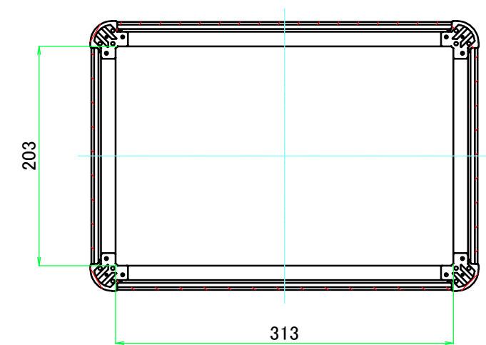
C-C (1:5)
