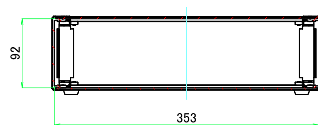
B-B (1:5)
