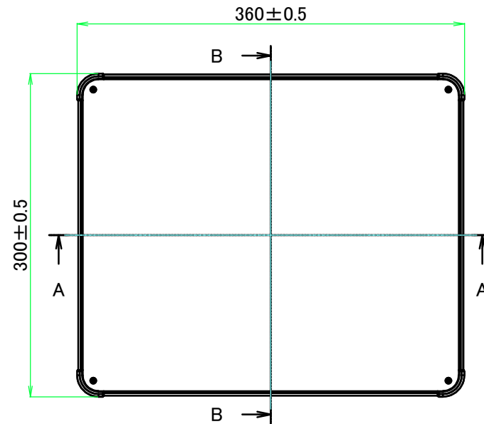
E view
