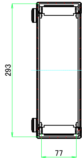
B-B (1:5)
