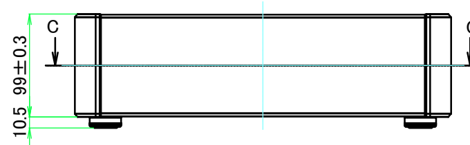
A view
