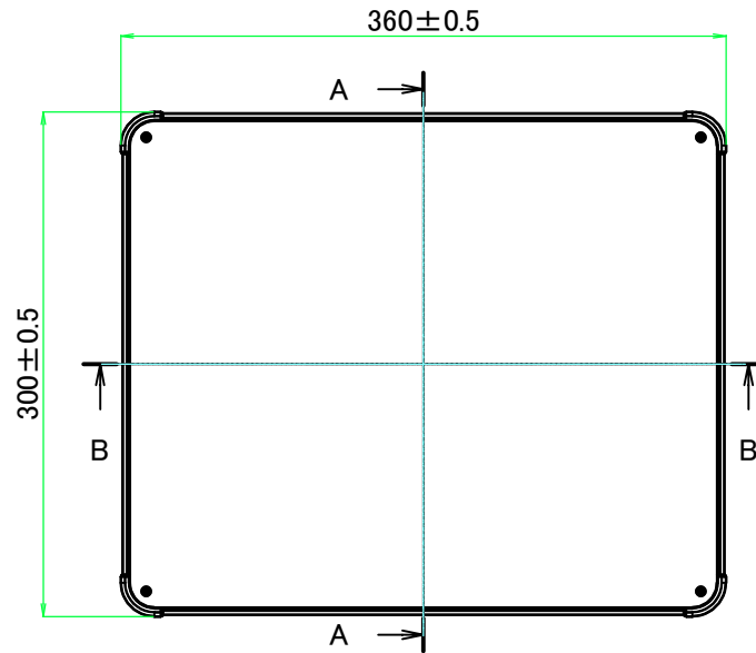
E view
