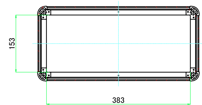
C-C (1:6)
