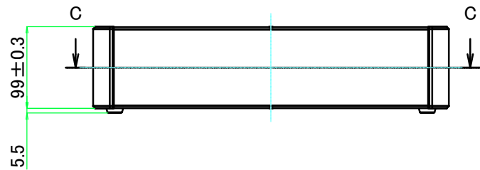
A view
