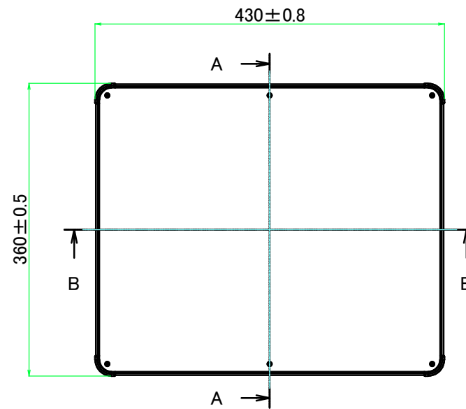
E view
