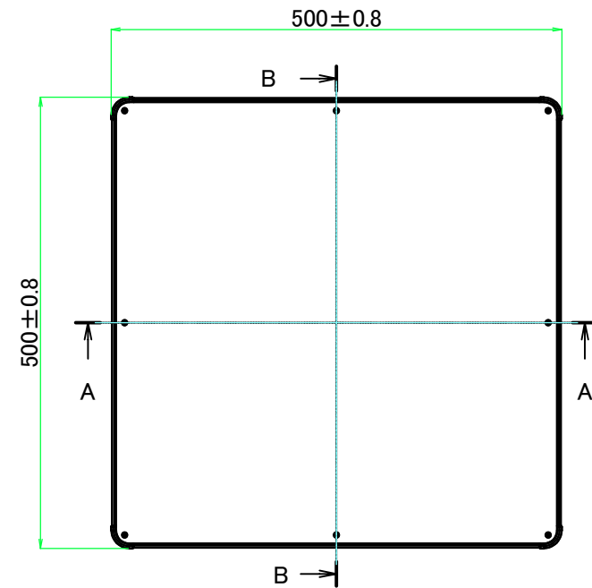
E view
