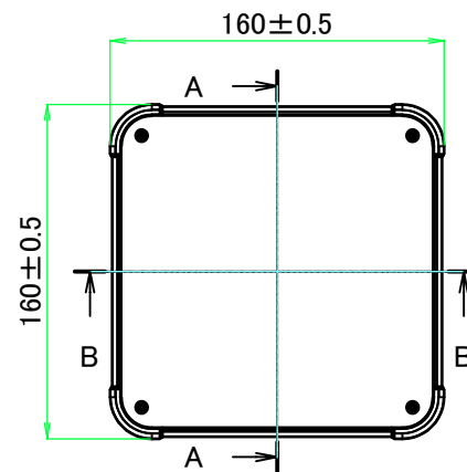
E view
