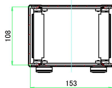
B-B (1:4)
