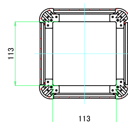
C-C (1:4)
