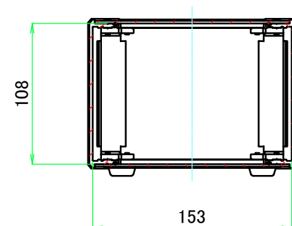
B-B (1:4)
