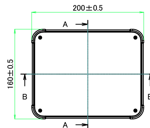
E view
