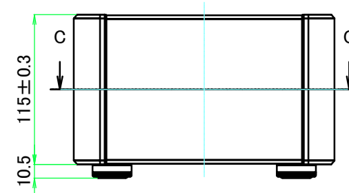
A view
