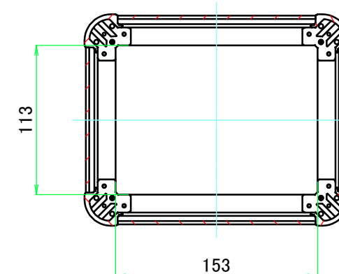
C-C (1:4)
