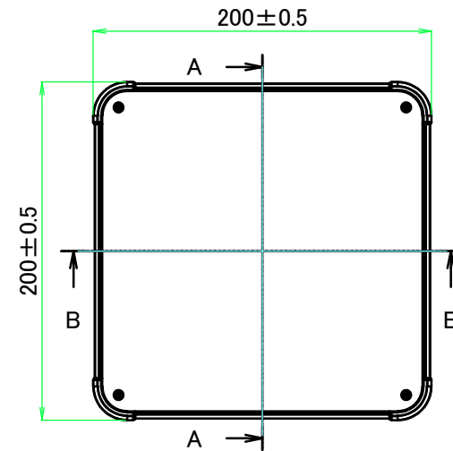
E view
