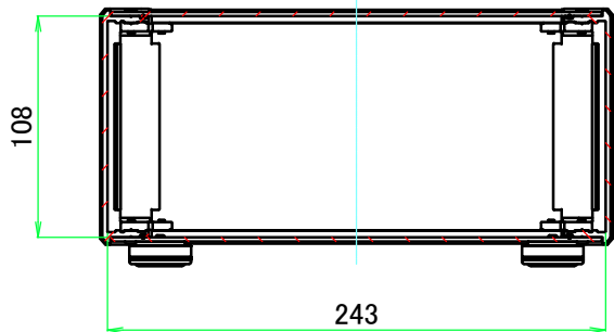
B-B (1:4)
