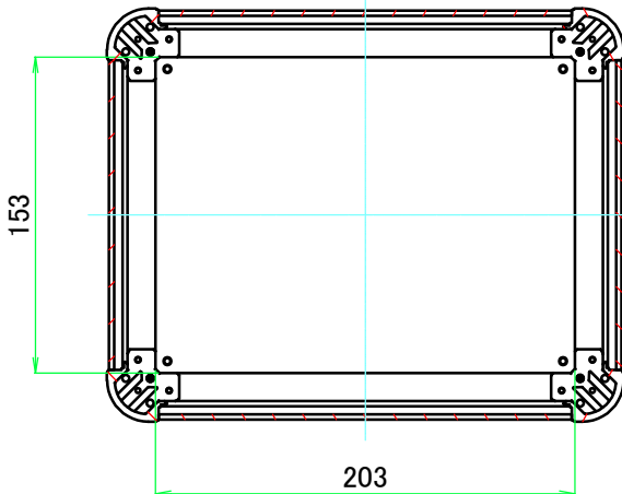
C-C (1:4)
