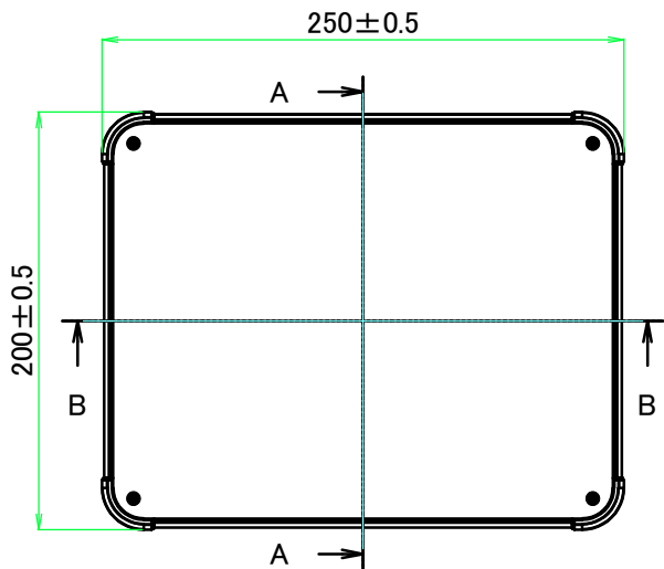
A view
