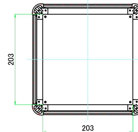
C-C (1:5)
