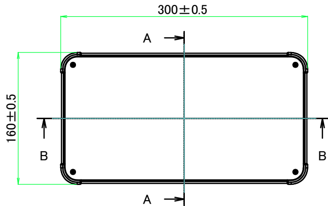
E view
