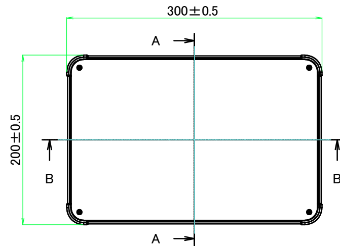
E view
