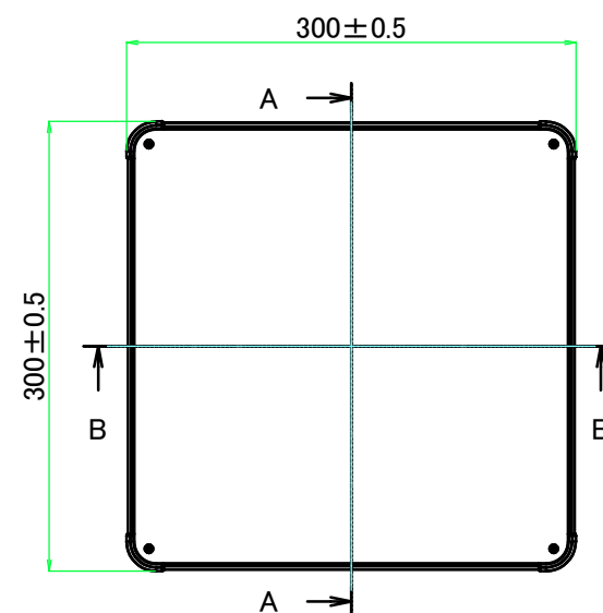
E view
