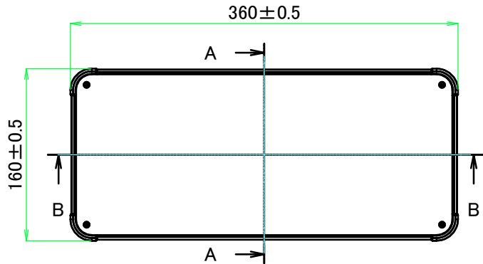
E view
