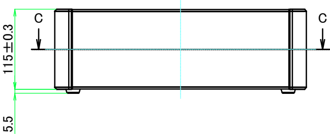
A view
