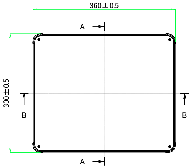
E view
