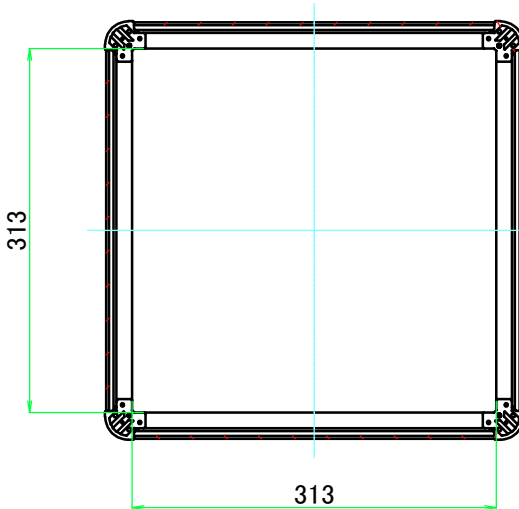
C-C (1:6.5)
