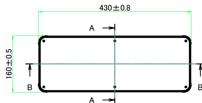
E view
