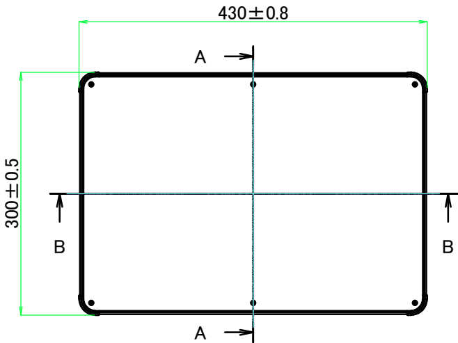
E view
