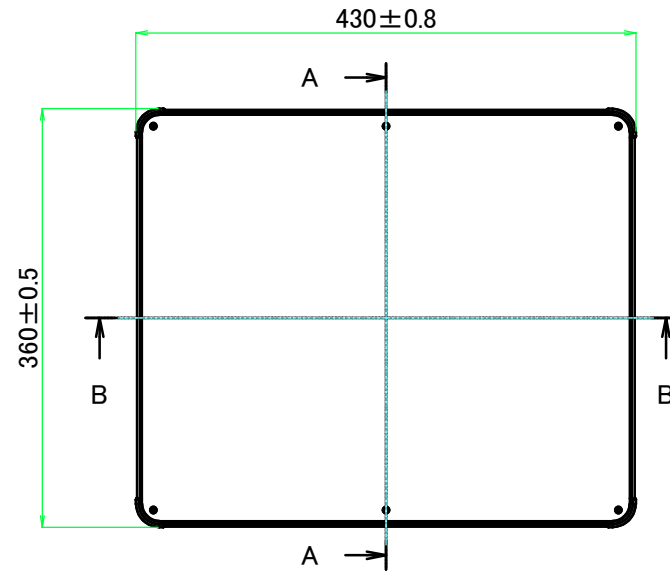
E view
