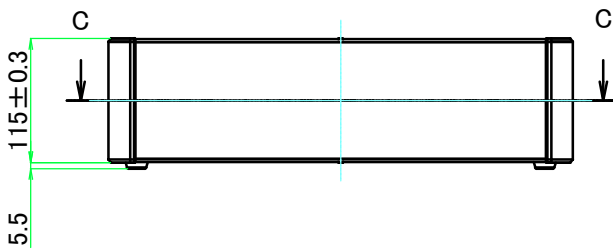
A view
