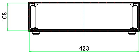
B-B (1:7)
