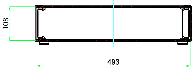
B-B (1:7)
