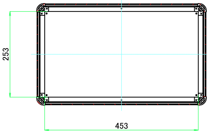
C-C (1:7)
