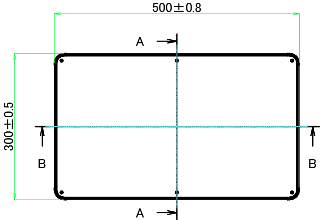
E view
