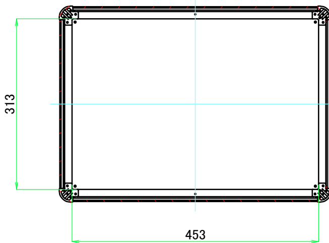
C-C (1:7)
