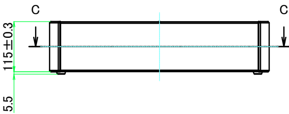
A view
