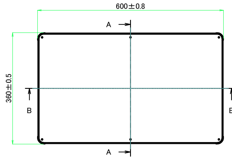
E view
