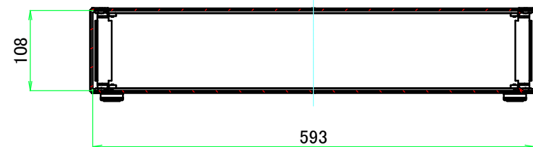
B-B (1:7)
