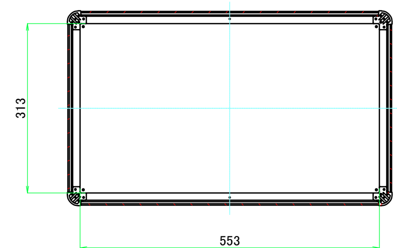
C-C (1:7)
