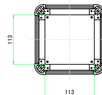
C-C (1:5)
