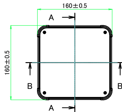
E view
