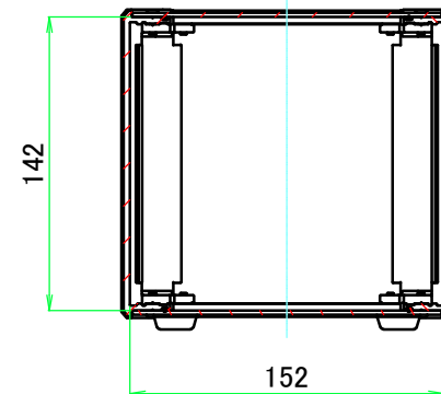
B-B (1:4)
