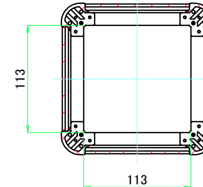
C-C (1:4)
