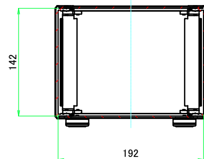
B-B (1:5)
