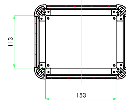
C-C (1:5)
