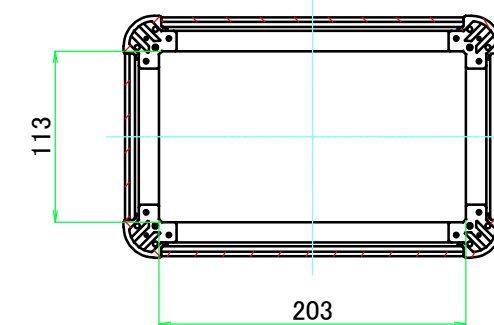
C-C (1:5)
