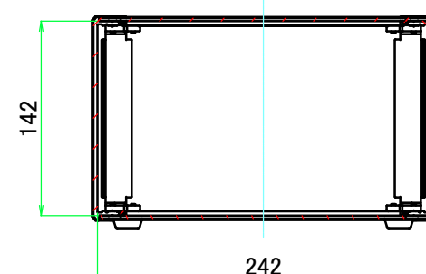
B-B (1:5)
