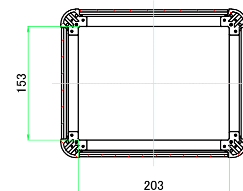
C-C (1:5)
