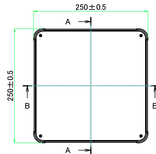
E view
