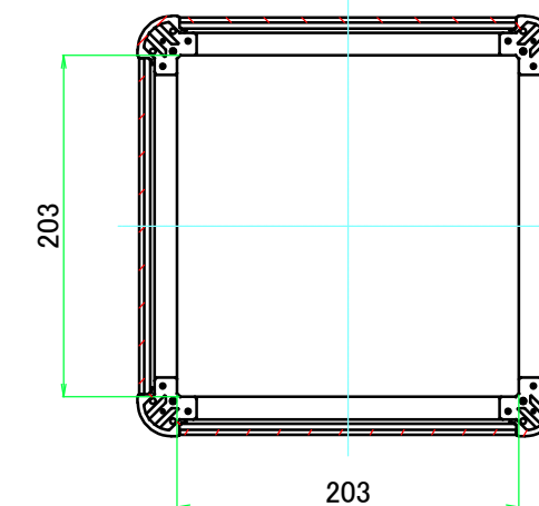
C-C (1:5)
