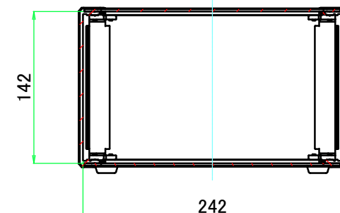
B-B (1:5)
