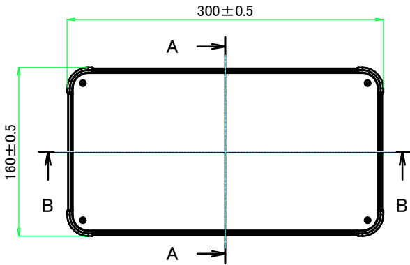
E view
