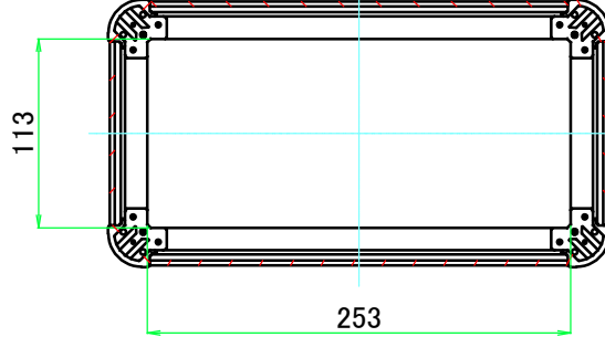
C-C (1:5)
