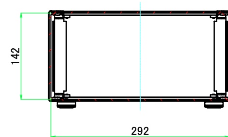
B-B (1:6)
