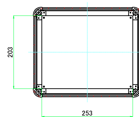
C-C (1:6)
