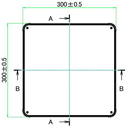
E view
