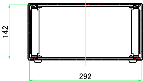
B-B (1:6)
