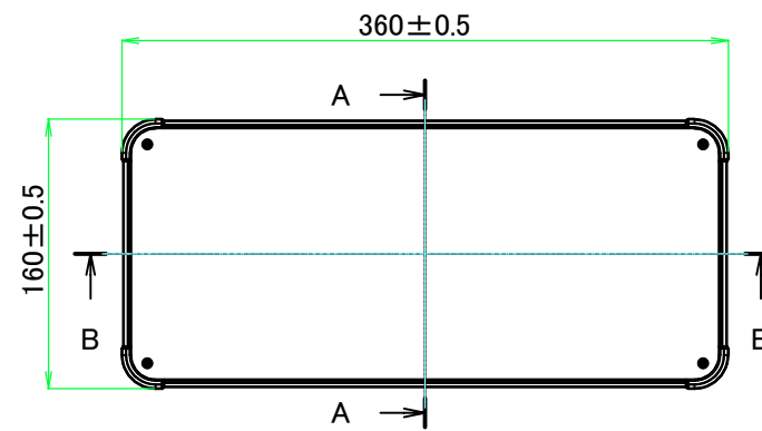
E view
