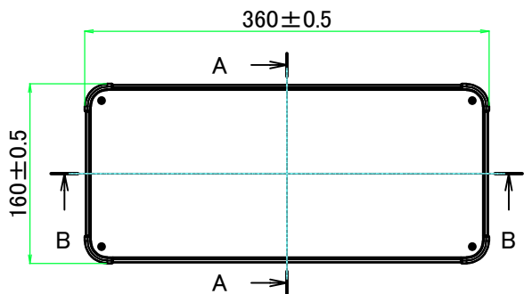
E view
