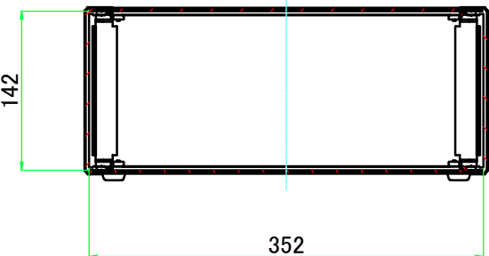
B-B (1:6)
