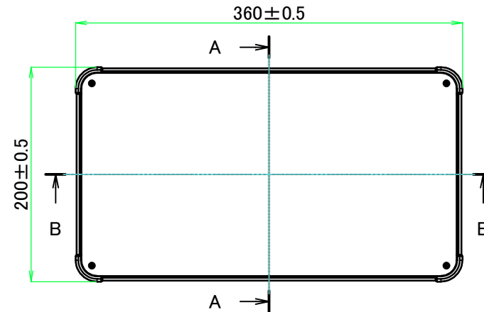
E view
