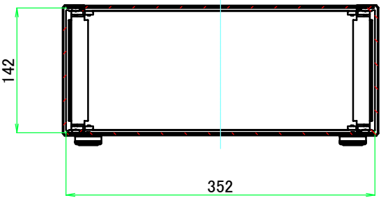
B-B (1:6)
