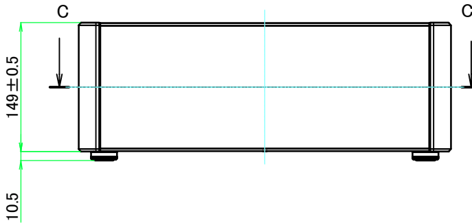
A view
