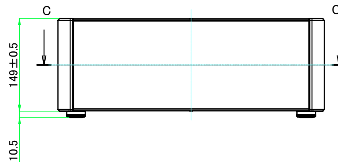
A view
