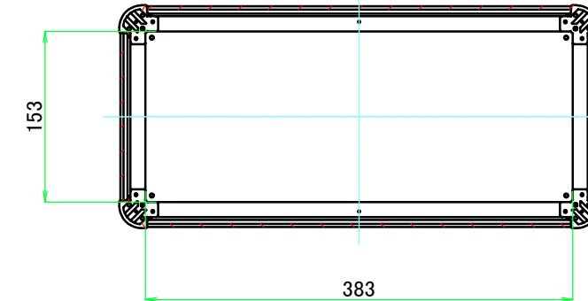
C-C (1:6)
