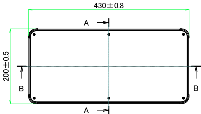
E view
