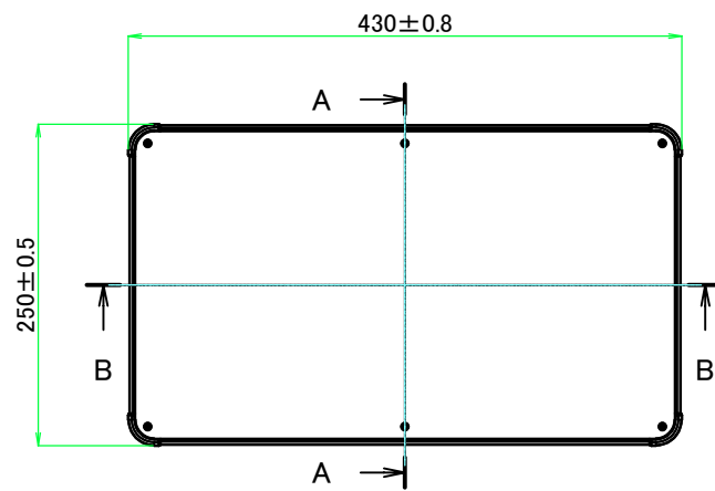
E view
