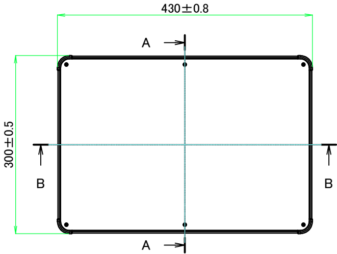
E view
